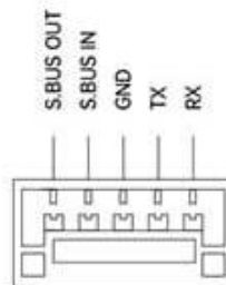
Gimbal Control
